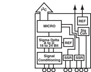
SMART MODULES WITH MULTICHANNEL INPUTS, AN ON-BOARD A TO D CONVERTER, MICROPROCESSOR, AND TWO SOLID STATE RELAY OUTPUTS
