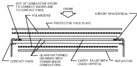
FIGURE 1. LCD Cross-Section
