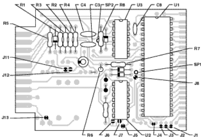
COMPONENT SIDE
