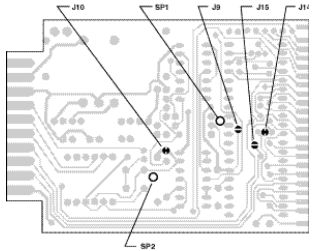
SOLDER SIDE
